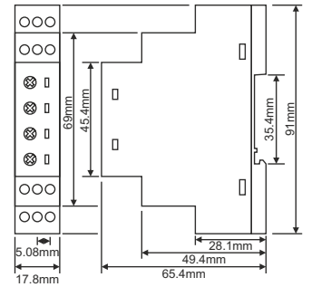
Dimensions for ERV-08M
