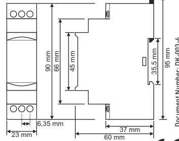
Dimensions for ERV-08
