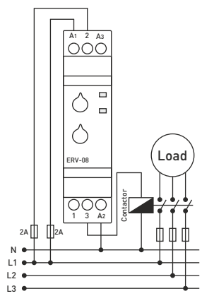
Connection diagram for ERV-08M
