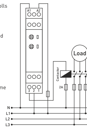
Connection diagram for ERV-08M
